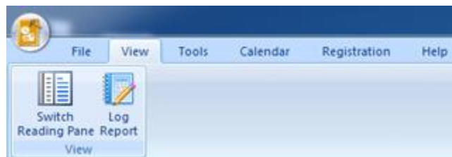
View Menu
