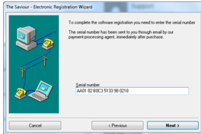
Registration Screen
